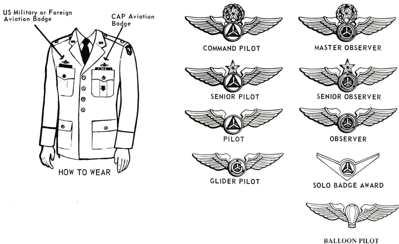
Figure 6-24. Aviation Badges.
